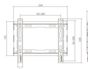
Dimensions (mm)
