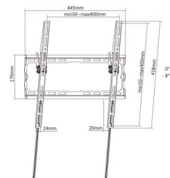
Dimensions (mm)
