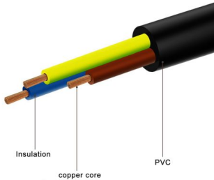
Copper 100% Inner conductor 0.75 mm 2 Cable Type: H05-VV-F30
