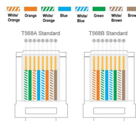
WIRING STRUCTURE
