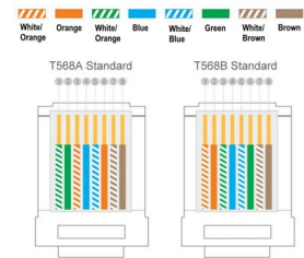
WIRING STRUCTURE
