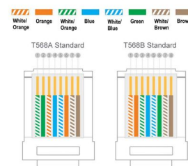
WIRING STRUCTURE
